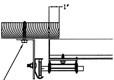
BRACKET MOUNT
